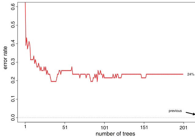
Figure 8. randomForest test set error for prostate cancer microarray study, now with training/test sets determined by early/late ID number. Results are much worse than in Figure 5. [Colour figure can be viewed at wileyonlinelibrary.com ]
