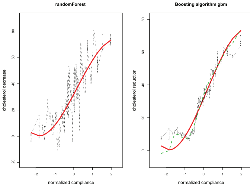
Figure 12. randomForest and gbm fits to the cholostyramine data of Figure 1 in Section 2. Heavy curve is cubic OLS; dashed curve in right panel is 8th degree OLS fit. [Colour figure can be viewed at wileyonlinelibrary.com ]
