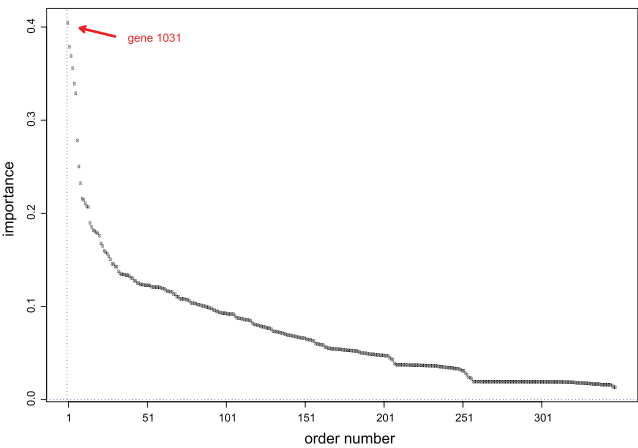
Figure 7. Random forest importance measures for prostate cancer prediction rule of Figure 5, plotted in order of declining importance. [Colour figure can be viewed at wileyonlinelibrary.com ]
