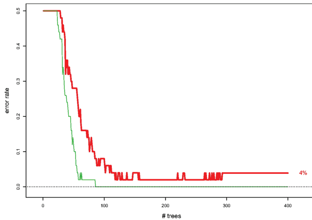
Figure 6. Test set error for boosting algorithm gbm applied to prostate cancer data. Thin curve is training set error, which went to zero at step 86. [Colour figure can be viewed at wileyonlinelibrary.com ]
