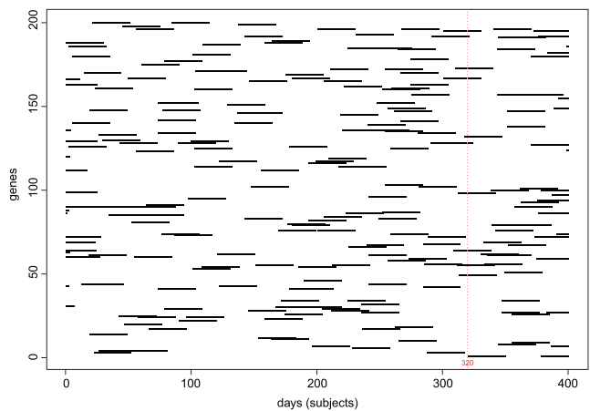
Figure 10. Black line segments indicate active episodes in the hypothetical microarray study. (Matrix transposed for typographical convenience.) [Colour figure can be viewed at wileyonlinelibrary.com ]
