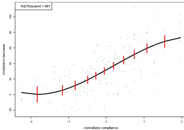
Figure 1. Black curve is OLS fitted regression to cholestyramine data (dots); vertical bars indicate \pm one standard error estimation. [Colour figure can be viewed at wileyonlinelibrary.com ]
