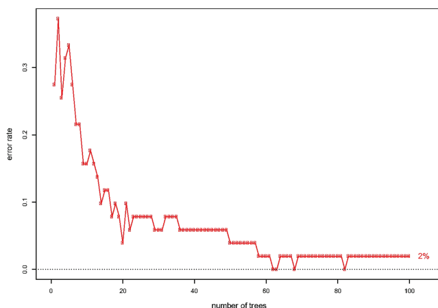
Figure 5. Test set error rate for random forests applied to prostate cancer microarray study, as a function of number of bootstrap trees. [Colour figure can be viewed at wileyonlinelibrary.com ]
