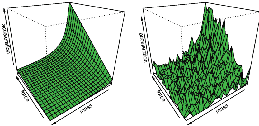
Figure 2. On left, a surface depicting Newton's second law of motion, \text{acceleration} = \text{force}/\text{mass} ; on right, a noisy version. [Colour figure can be viewed at wileyonlinelibrary.com ]
