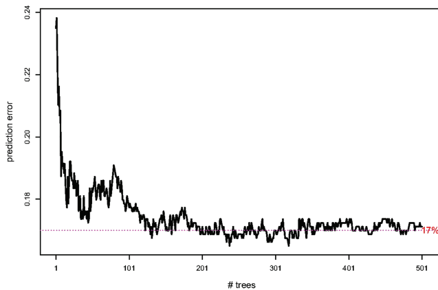
Figure 4. Random forest prediction error rate for neonate data, as a function of number of bootstrapped trees; it has cross-validated error rate 17%. [Colour figure can be viewed at wileyonlinelibrary.com ]
