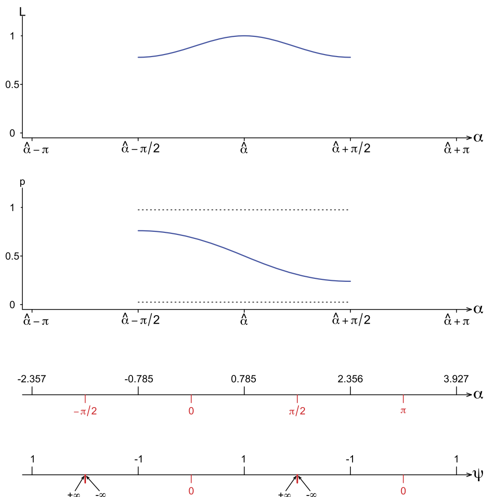
FIG. 3. The significance function and likelihood function for example B, ( y_1 = 0.5 , y_2 = 0.5 ). The maximum likelihood estimate is \hat{\alpha} = 0.785 and we show both the \alpha and \psi scale for the parameter. There are discontinuities in \psi , at \alpha = \pm\pi/2 , where y_1 changes from positive to negative. Confidence intervals for \alpha are only available for a restricted range of confidence levels, (0.24, 0.76) . For other confidence levels all values of \alpha and all values of \psi are consistent with the data. Horizontal dotted lines are drawn at p = 0.975 and p = 0.025 .
