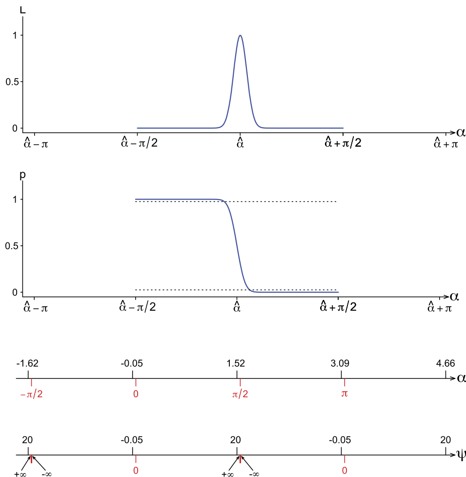
FIG. 2. The significance function and likelihood function for example, A: y_1 = 0.5 , y_2 = 10 . The maximum likelihood estimate is \hat{\alpha} = 1.52 and we show both the \alpha and \psi scale for the parameter. There are two discontinuities in \psi shown, at \alpha = \pm\pi/2 , where y_1 changes from positive to negative. The discontinuity at \pi/2 leads to what Fieller (1954) called exclusive confidence regions for \psi at confidence level 0.95. Horizontal dotted lines are drawn at p = 0.975 and p = 0.025 .
