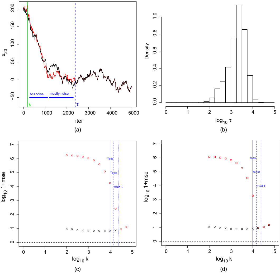
Fig. 9. Plots from the experiment described in the text: (a) first 5000 iterations of the first simulation ( t ; \tau ; k , putative k ); (b) histogram of all 5000 values of \log_{10}(\tau) ; (c) \log_{10}(1 + \text{MSE}) (mean taken over the 5000 simulations) of unbiased MCMC ( \circ ) and MCMC ( \times ) sampling as a function of k ( l , \tau_{0.99} ; \dagger , \tau_{0.999} ; \ddagger , largest \tau (not \tau_{\max} ) value over the 5000 simulations); (d) \log_{10}(1 + \text{MSE}) of Rao–Blackwellized unbiased MCMC ( \square ) and MCMC ( \times ) as a function of k
